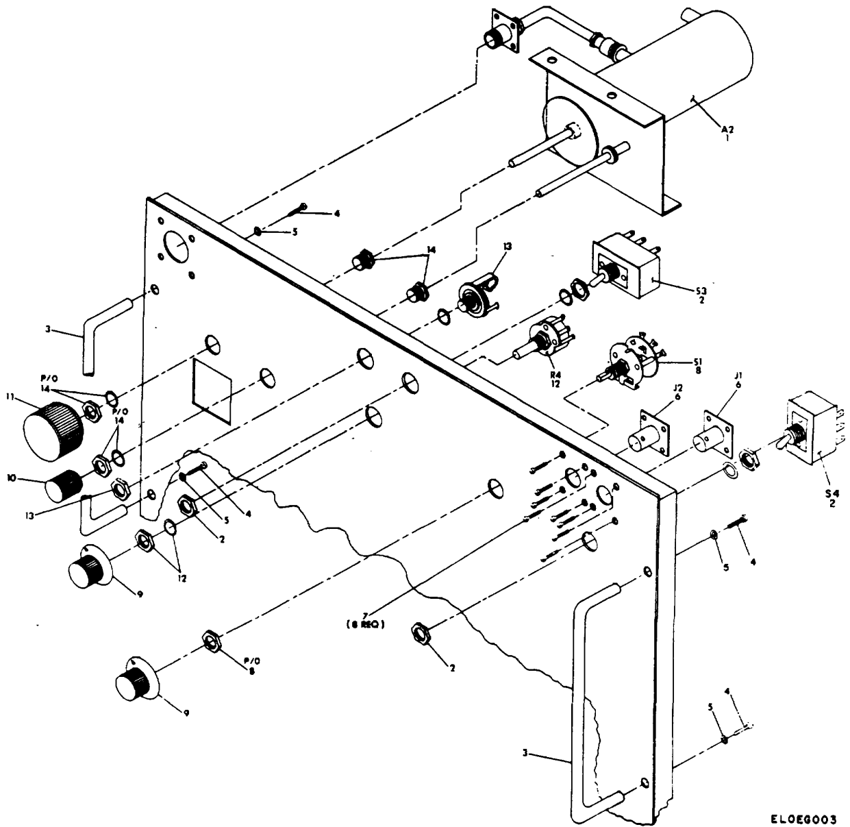
Figure 3. Front Chassis Assembly.
