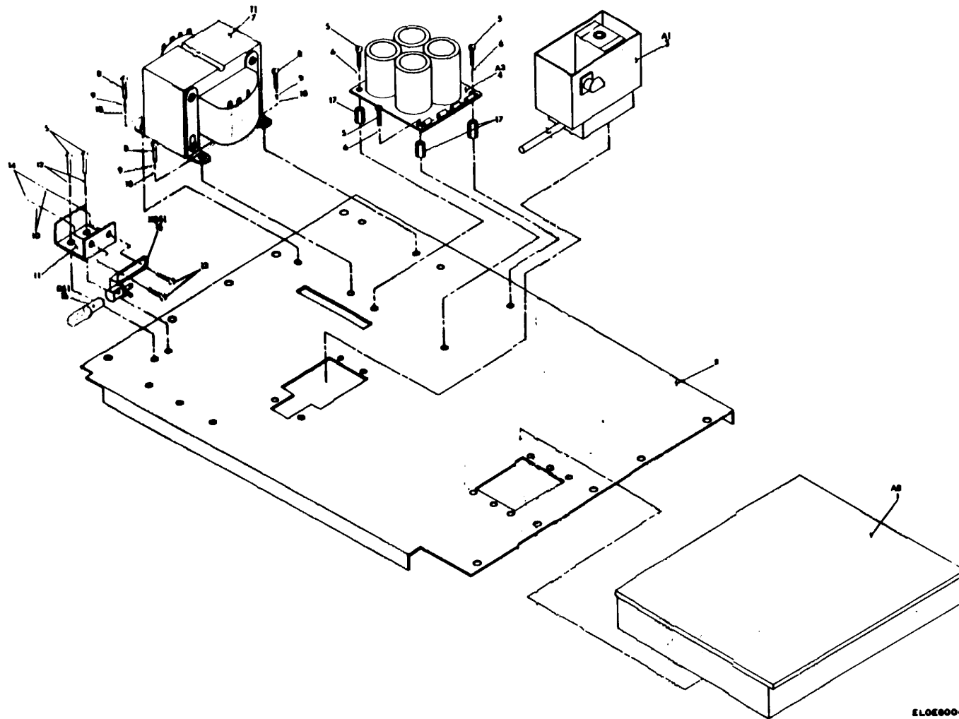
Figure 4. Bottom Chassis Assembly.
