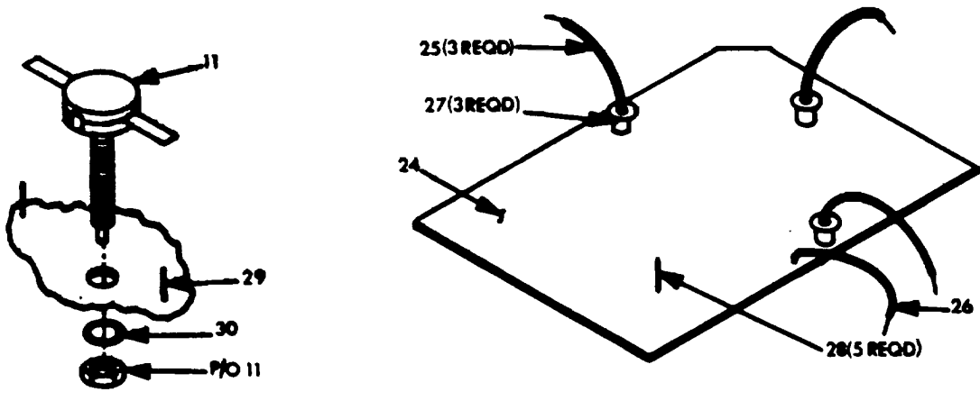
Figure 16. Circuit Card Assembly (A9A2).
