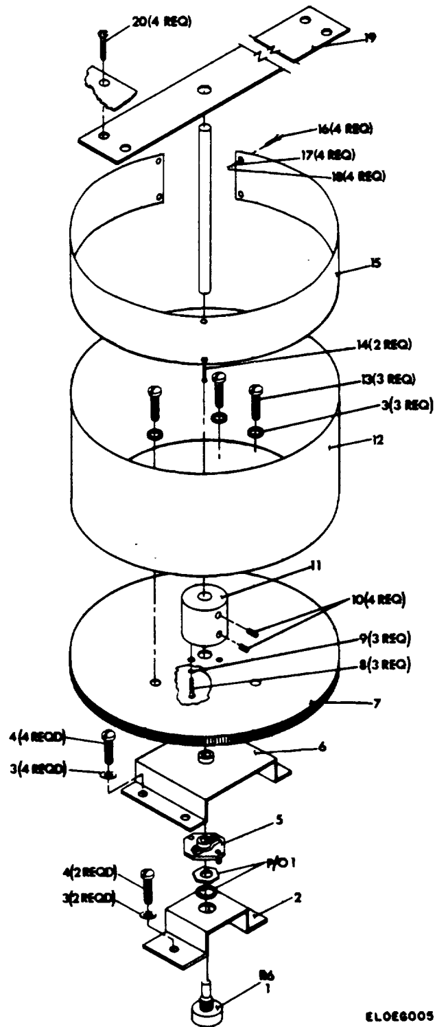
Figure 5. Drum Assembly. 23
