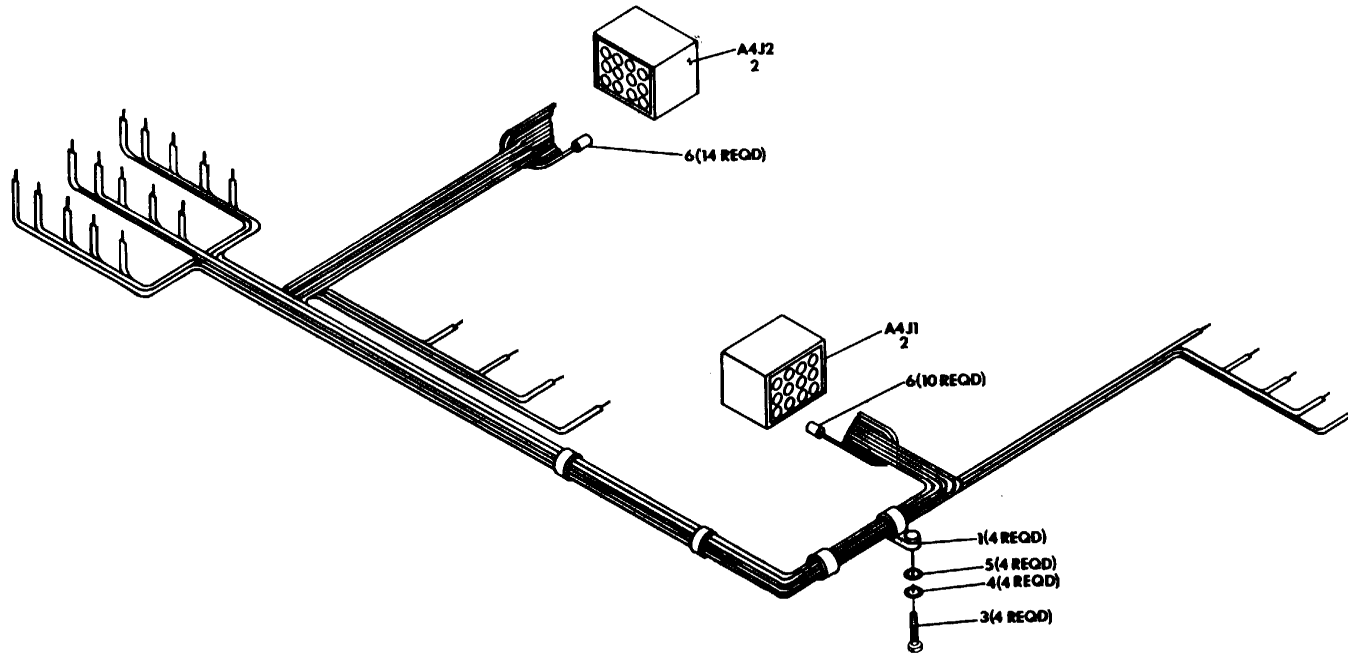
Figure 10. Harness Assembly. 28
