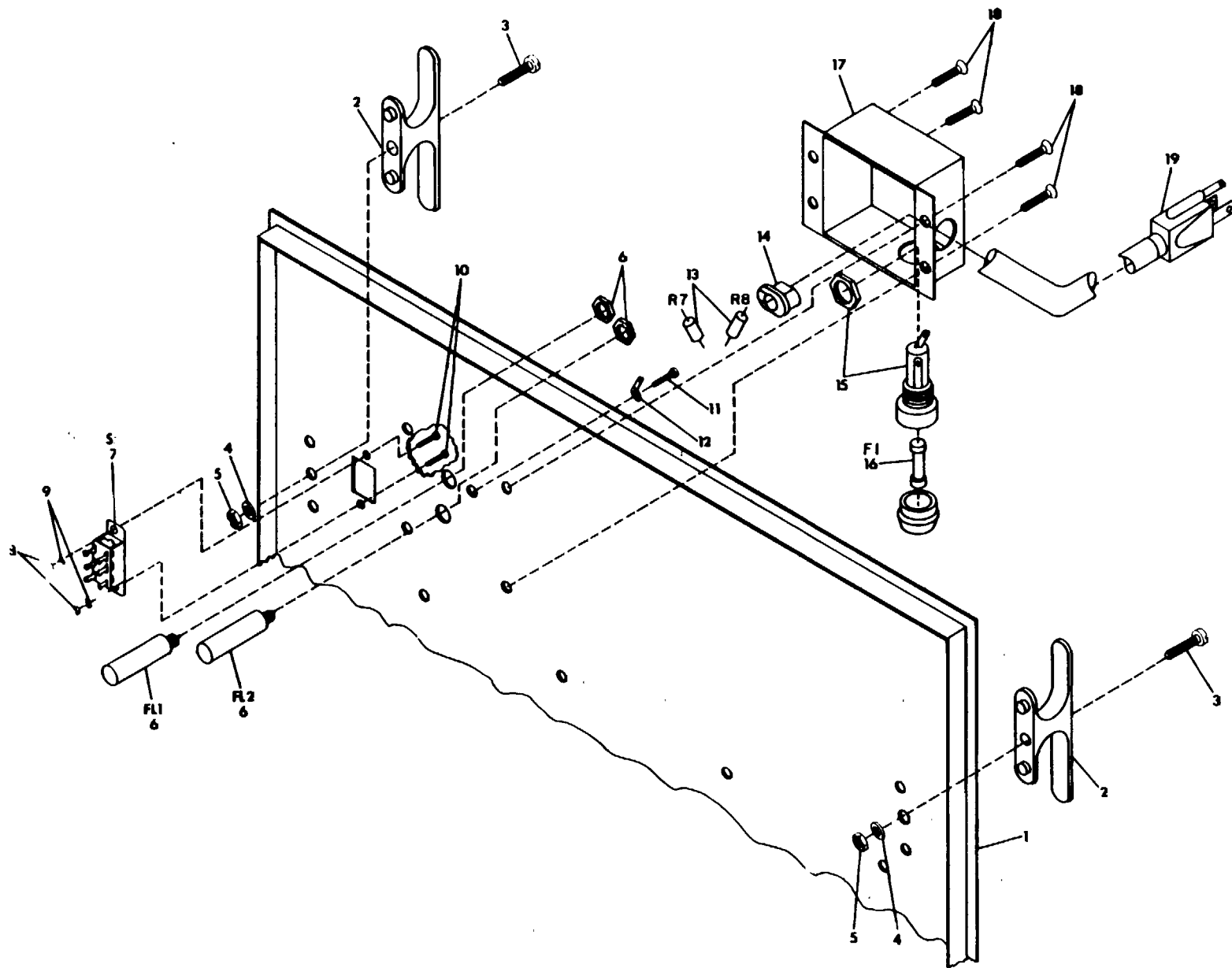
Figure 2. Rear Chassis Assembly. 20
