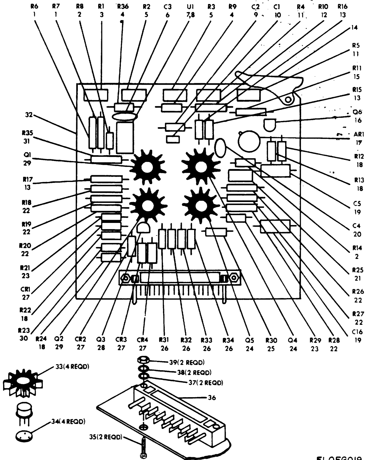
Figure 19. Circuit Card Assembly (A7).
