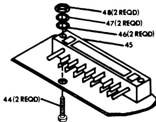
Figure 18. Circuit Card Assembly (A5).
