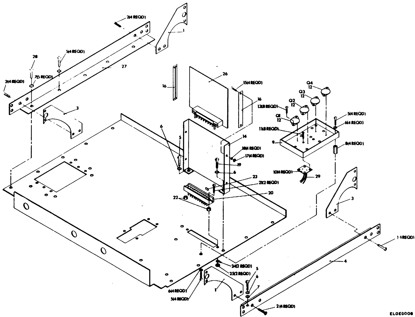
Figure 8. Top Chassis Assembly. 26
