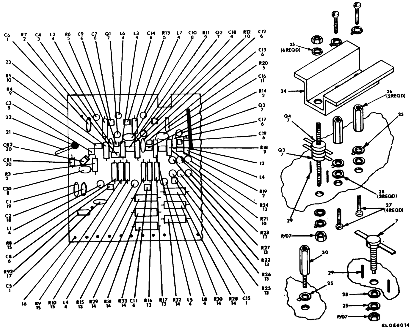
Figure 14. Circuit Card Assembly, Left (A9A1)
