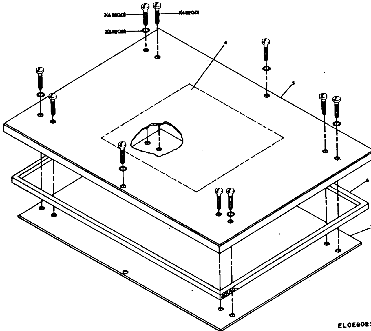
Figure 22. Cover Assembly (P/O A8).
