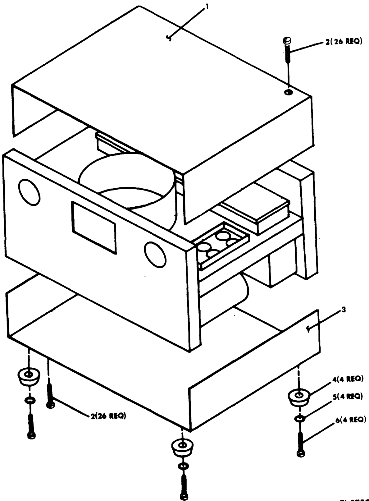
Figure 1. Cover Assembly (Top and Bottom).
